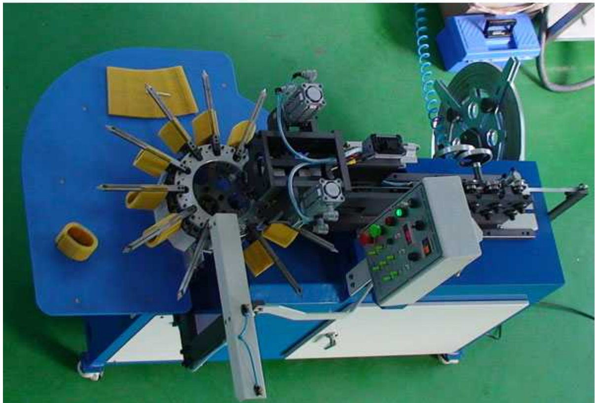
MAIN M/C PHOTO
