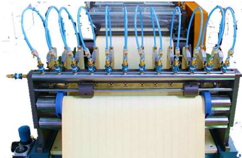
SLITTING DEVICE
